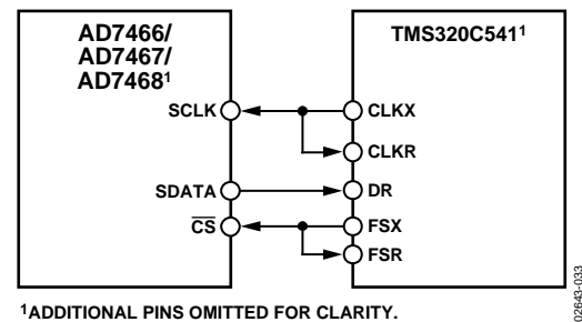
Figure 32. Interfacing to the TMS320C541
