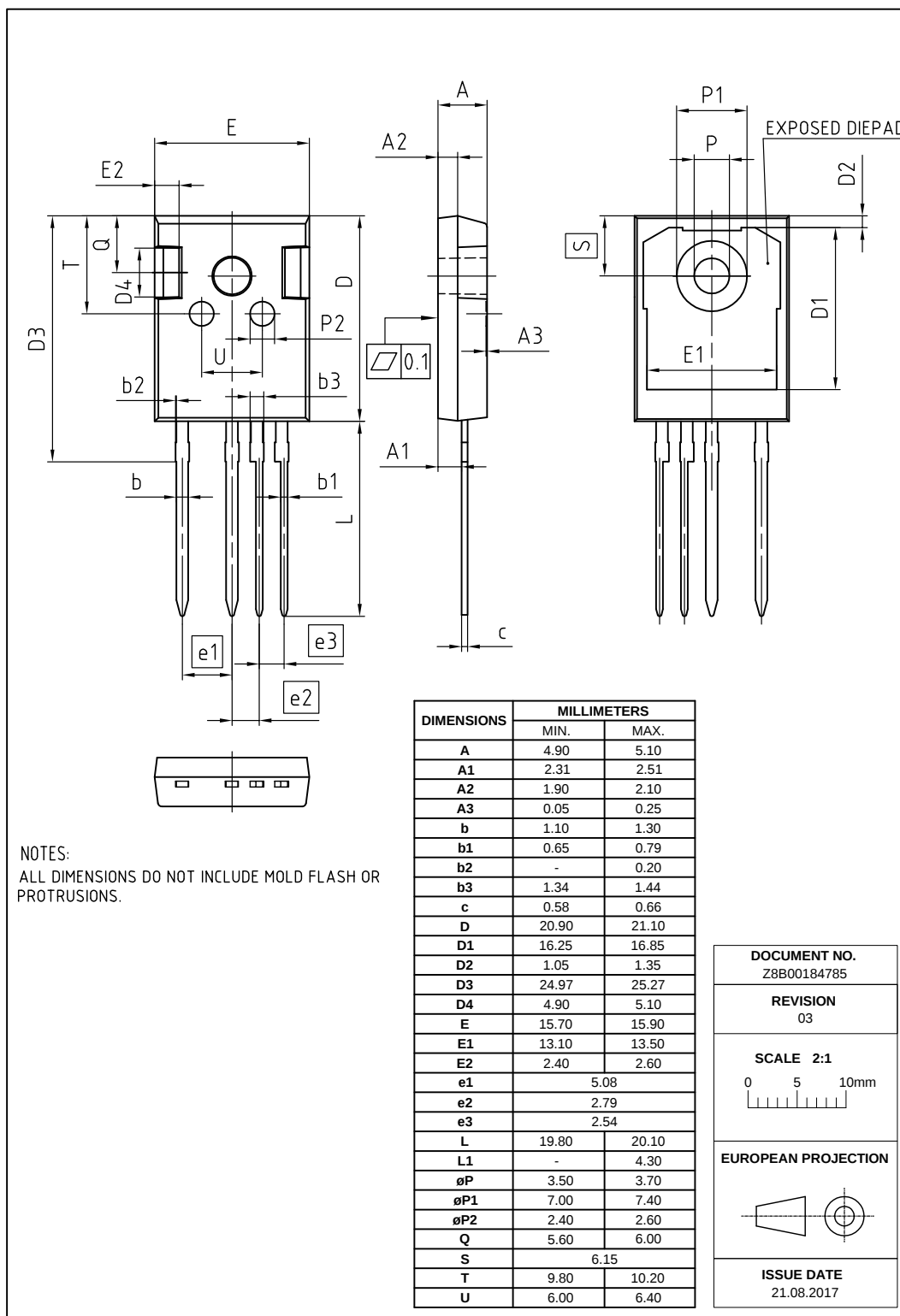
Figure 1 Outline PG-TO 247-4-3, dimensions in mm - Industrial Grade
