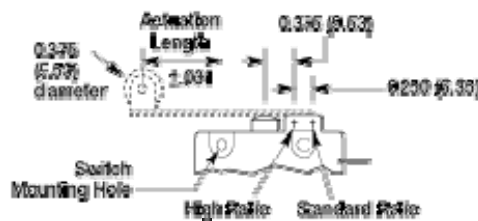
Roller Actuator Version (-00K and -50K)
