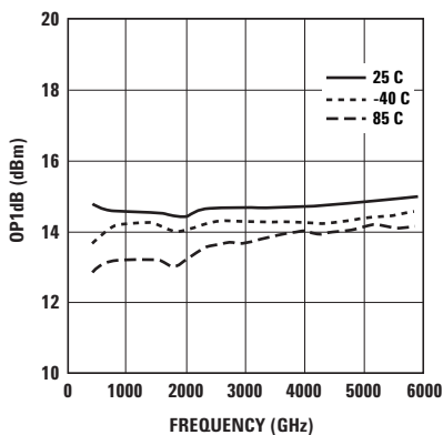
Figure 15. OP1dB vs. Frequency (3V 20 mA).
