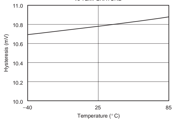
SIGN COMPARATOR HYSTERESIS vs TEMPERATURE
