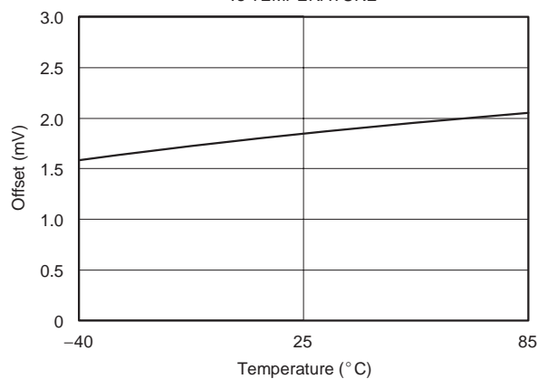
SIGN COMPARATOR OFFSET vs TEMPERATURE
