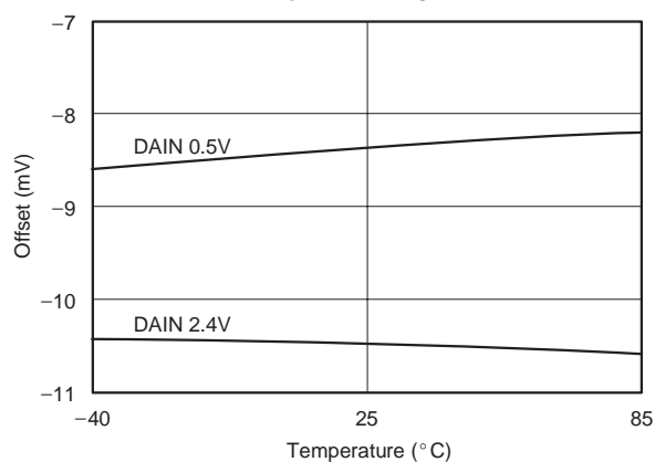
WINDOW COMPARATOR OFFSET vs TEMPERATURE
