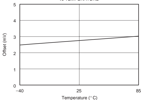
ENCODER COMPARATOR OFFSET vs TEMPERATURE
