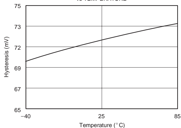
ENCODER COMPARATOR HYSTERESIS vs TEMPERATURE
