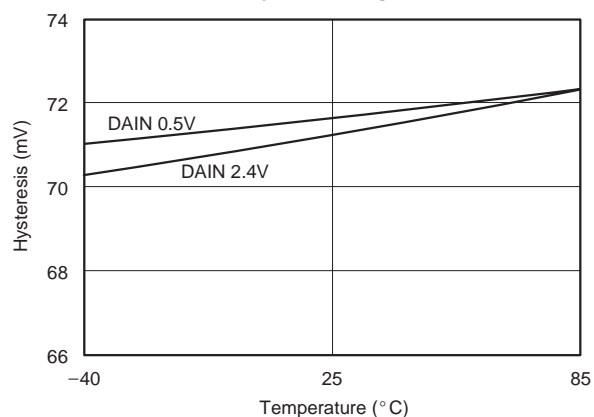
WINDOW COMPARATOR HYSTERESIS vs TEMPERATURE
