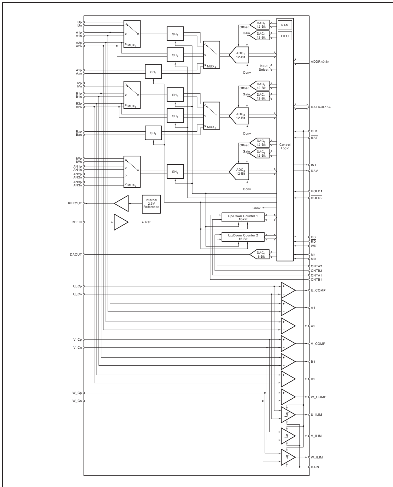
Figure 1–2. Functional Diagram
