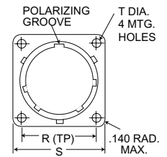
RECEPTACLE ASSEMBLY
