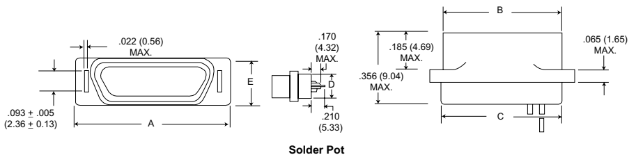
Solder Pot
