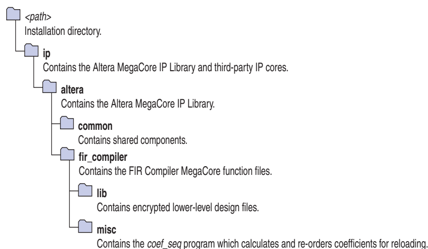
Figure 1-4. Directory Structure
