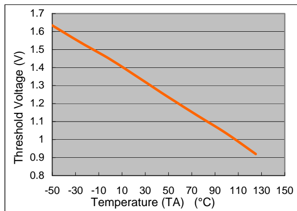
AP1509 Threshold Voltage vs. Temperature ( V_{IN}=12V , I_o=100mA )
