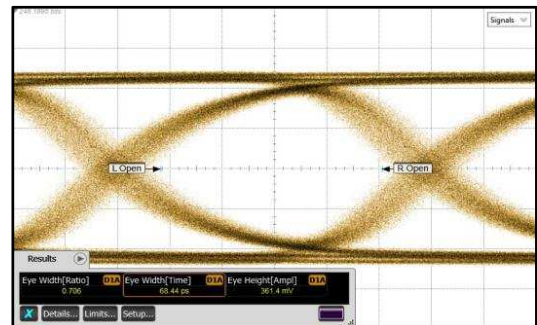
Figure 28. TL = 7-Meter 30-AWG 100 \Omega Twin-Axial Cable, DS100BR210 CHA, 10.3125 Gbps
