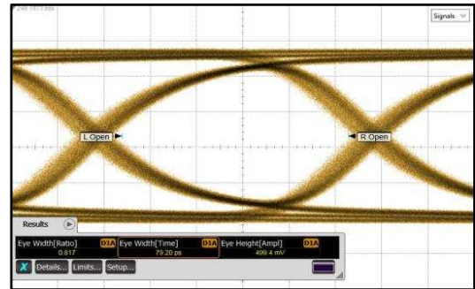
Figure 26. TL = 3-Meter 30-AWG 100 \Omega Twin-Axial Cable, DS100BR210 CHA, 10.3125 Gbps
