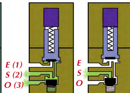
Normally-Open 3-Way Valve
