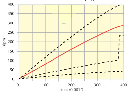
Characteristic Curve Flow Rate @ 100 psig
