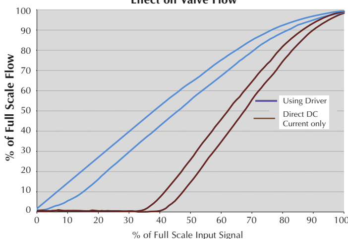
Figure 1: Effect of Driver Output on EVP Flow
