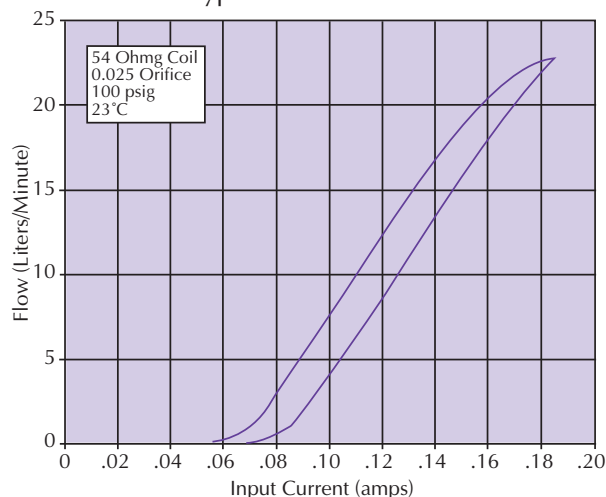
Typical Performance
