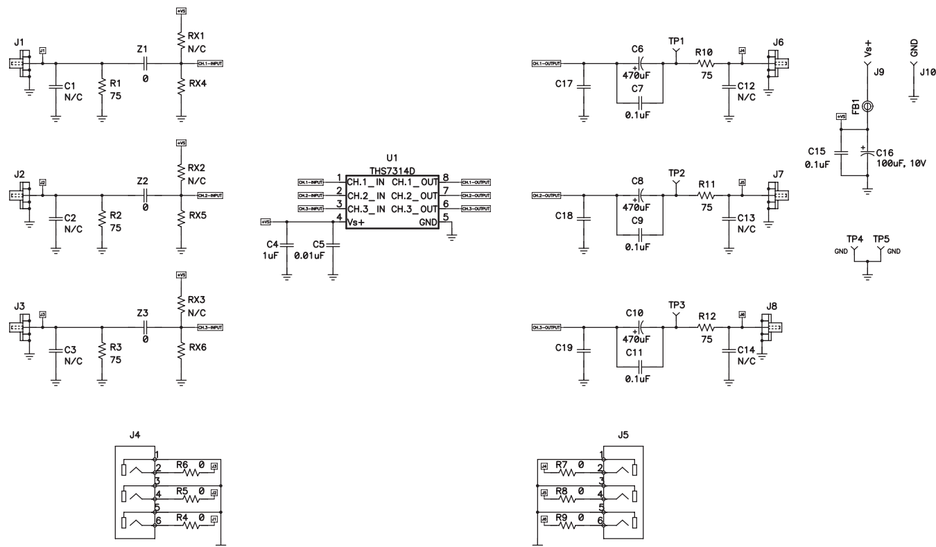
Figure 35. THS7314 Schematic
