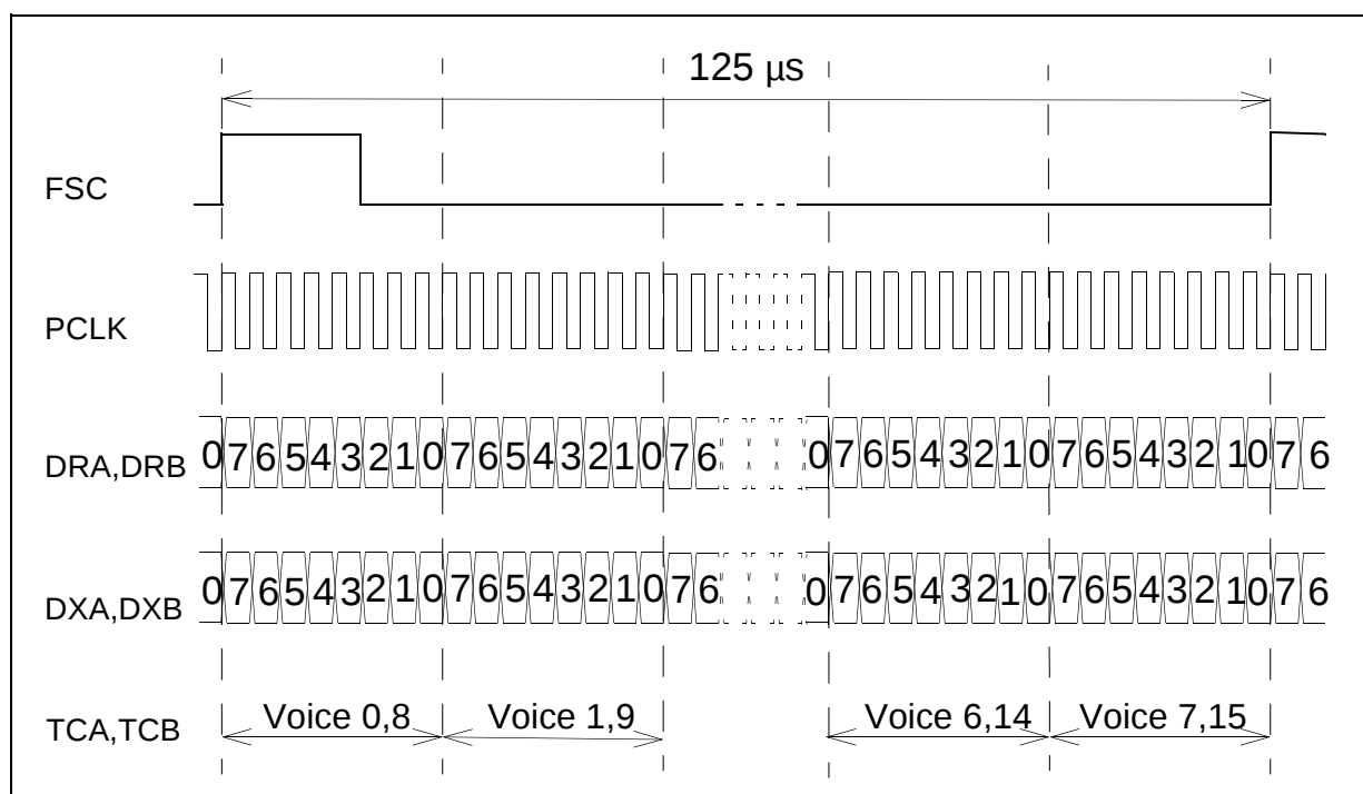
Figure 16 Example for Single Clock Rate, 512 kb/s
