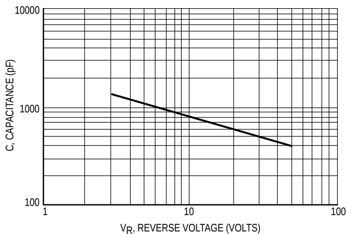
Figure 3. Typical Capacitance Per Leg
