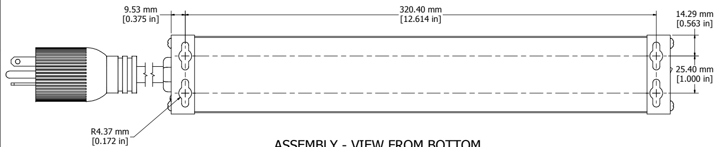
ASSEMBLY - VIEW FROM BOTTOM
