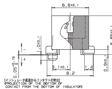
SECT. B-B
