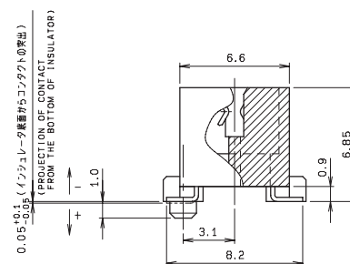
SECT. B-B
