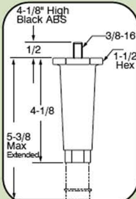
8540 ADJUSTABLE LEG
