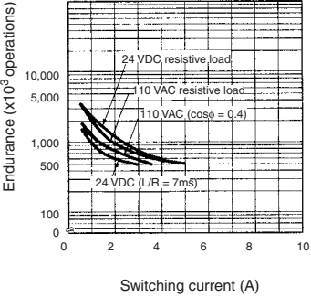
LY2Z Endurance
