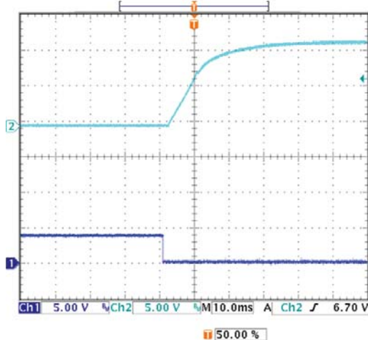
On/Off Enable delay (Vin=48V, Vout=nom, Iout=17A, Load=6000μF, Ta=+25°C) Ch1=Enable, Ch2= Vout
