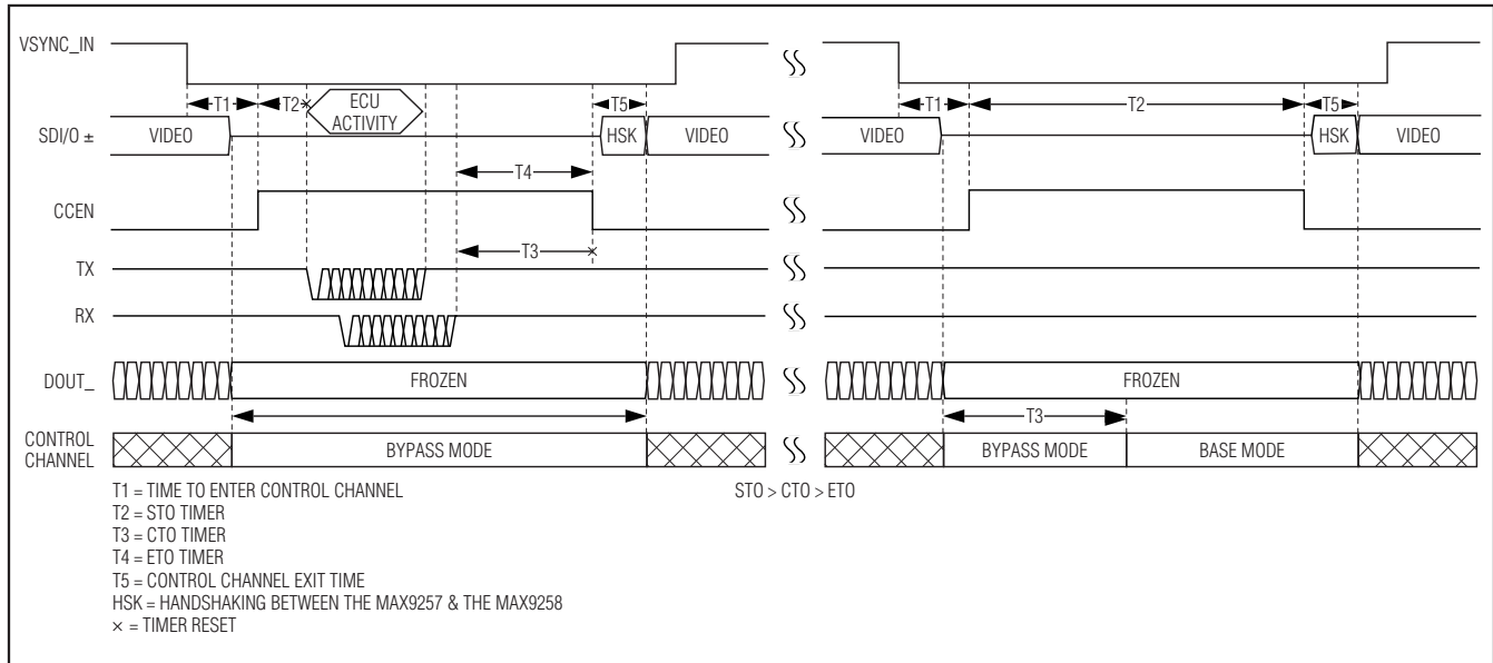
Figure 24. CTO Timing
