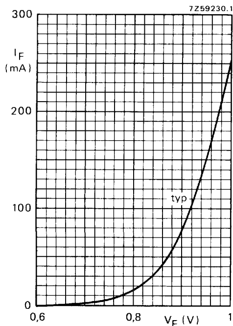
Fig. 12 T_j = 25\text{ }^{\circ}\text{C} .
