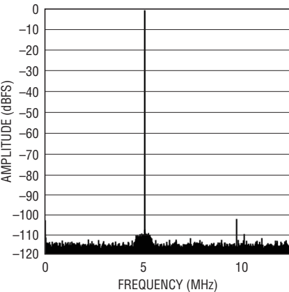
LTC2190: 64k Point FFT, f_{IN} = 5\text{MHz} , -1dBFS, 25Msps
