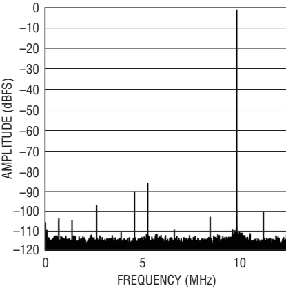
LTC2190: 64k Point FFT, f_{IN} = 140\text{MHz} , -1dBFS, 25Msps
