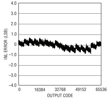
LTC2190: Integral Nonlinearity (INL)
