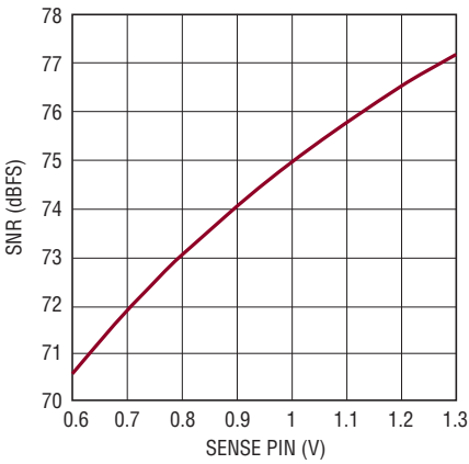
LTC2191: SNR vs SENSE, f_{IN} = 5\text{MHz} , -1dBFS
