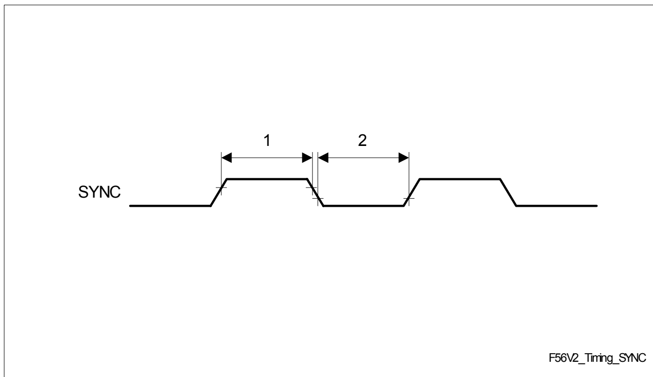
Figure 107 SYNC Timing
