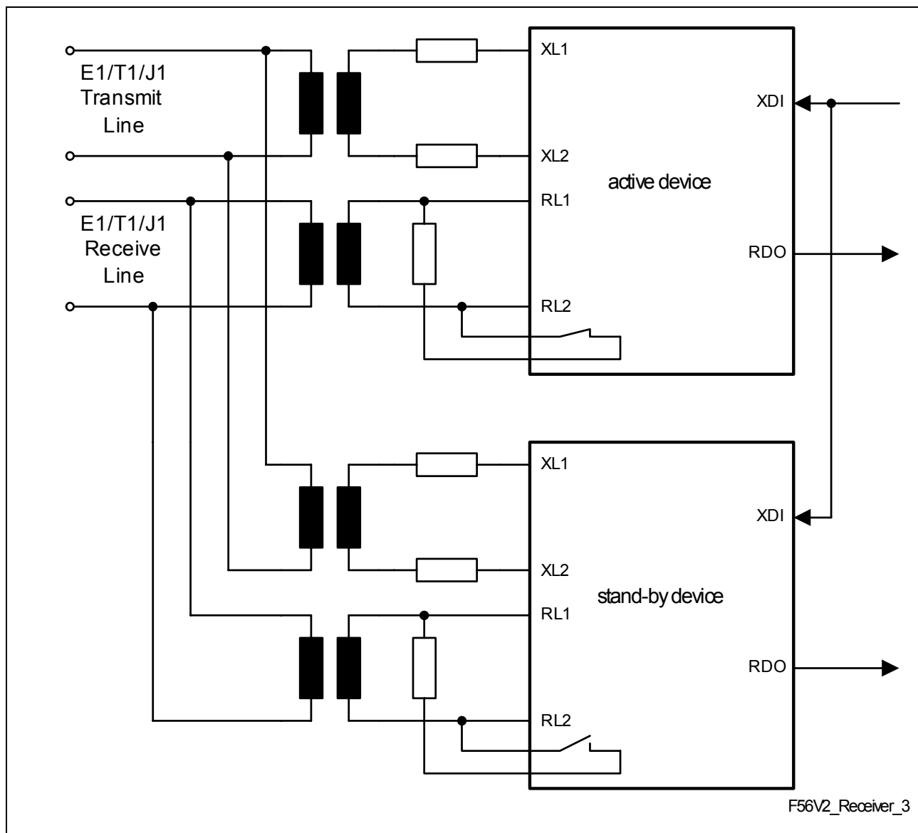
Figure 49 Long Haul Protection Switching Application (T1/J1)
