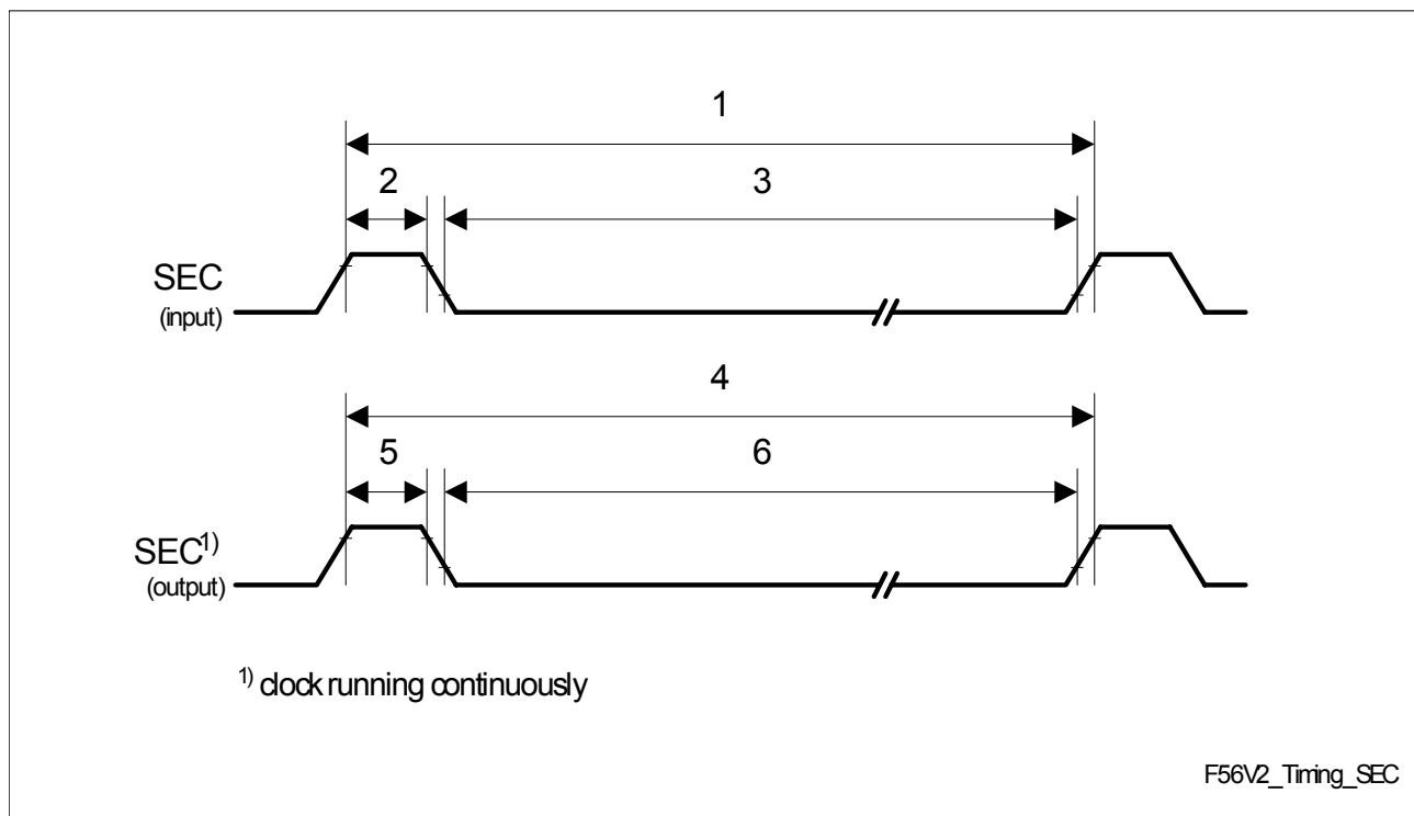
Figure 105 SEC Timing
