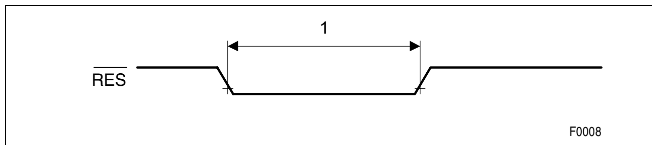
Figure 88 Reset Timing
