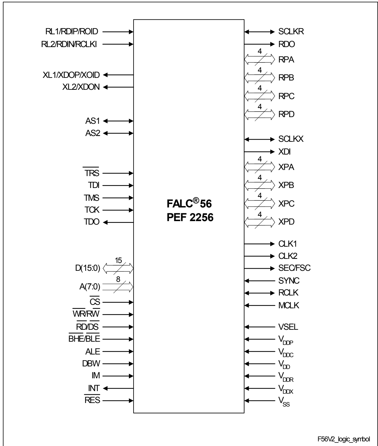
Figure 3 Logic Symbol
