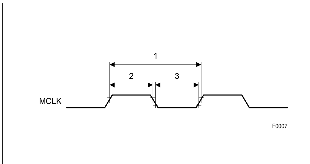
Figure 86 MCLK Timing
