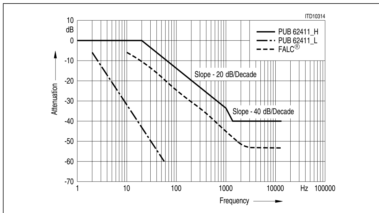
Figure 50 Jitter Attenuation Performance (T1/J1)
