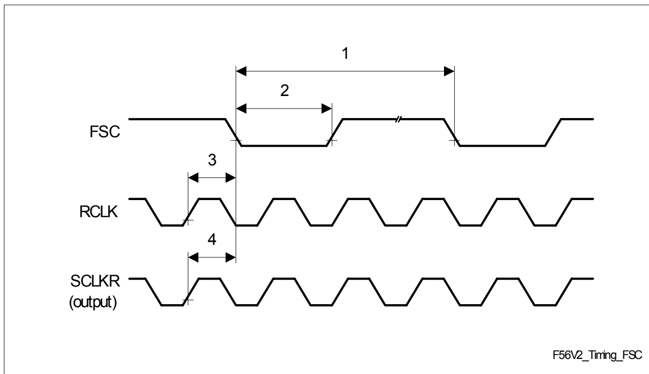
Figure 106 FSC Timing
