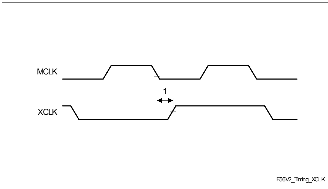
Figure 104 XCLK Timing
