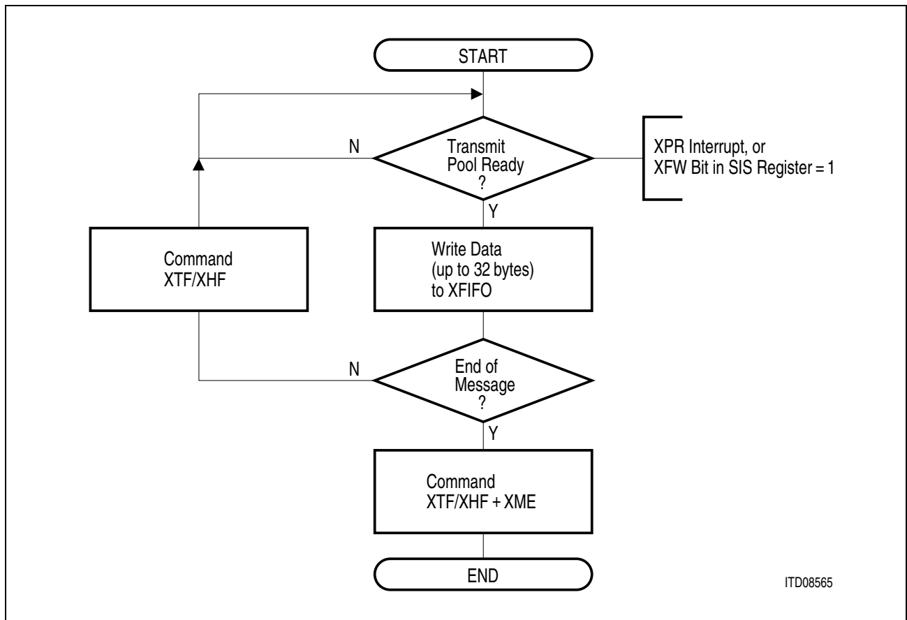
Figure 83 Interrupt Driven Data Transmission (flow diagram)
