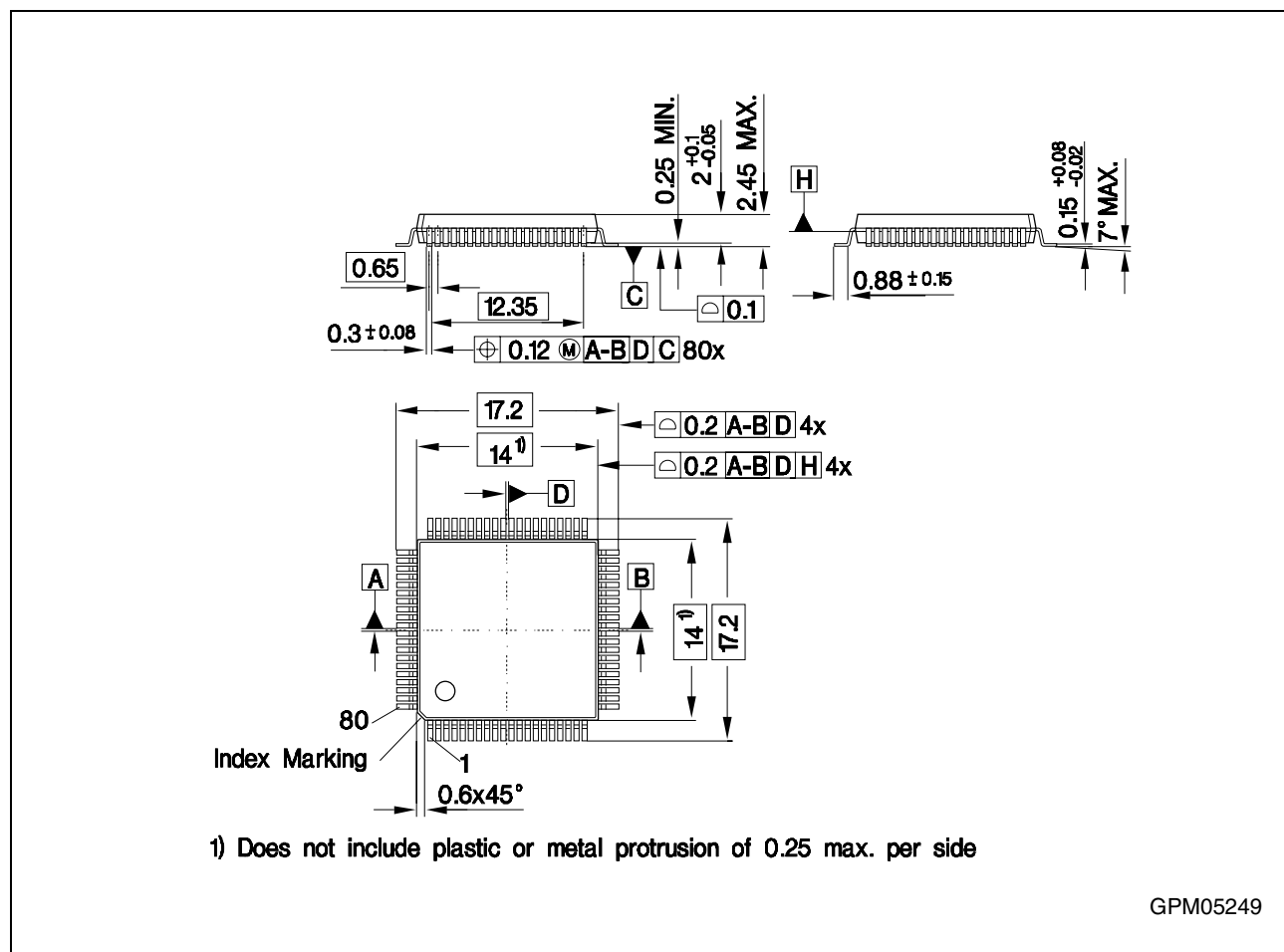
Figure 114 P-MQFP-80-1 (Plastic Metric Quad Flat Package)
