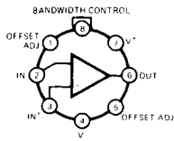
(outline dwg TO-99)
