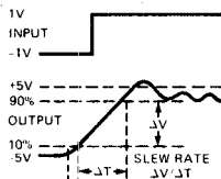
SLEW RATE
