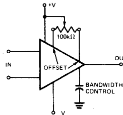
SUGGESTED OFFSET ZERO ADJUST AND BANDWIDTH CONTROL HOOK-UP
