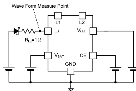
< Circuit No.⑥ >
