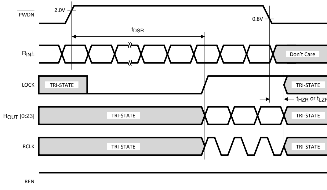
Figure 5-14. Deserializer PLL Lock Times and RPWDB Tri-State Delay
