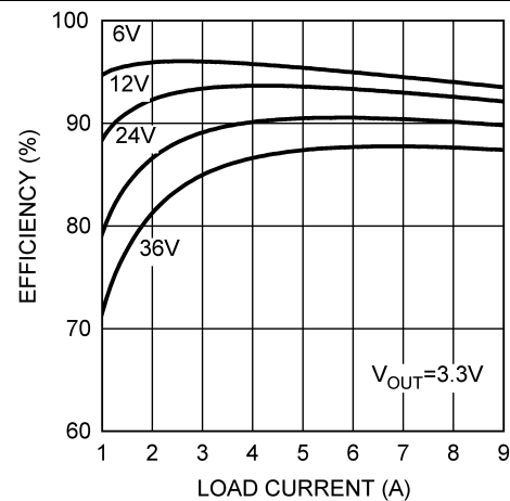
Figure 34. Typical Efficiency vs Load Current
