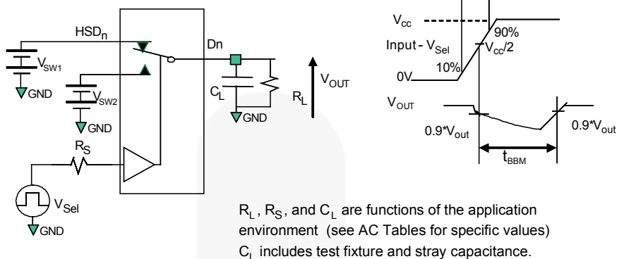
Figure 9. Break-Before-Make Interval Timing
