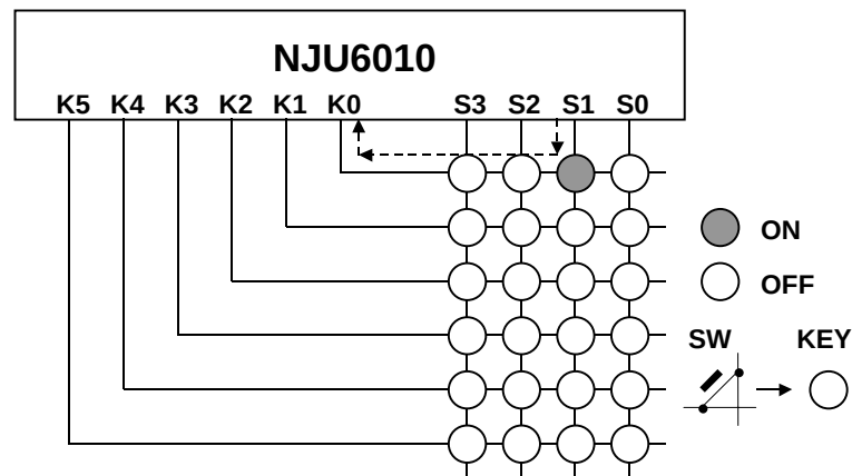
Fig. 3 Key-scan Checking (Example 1)
