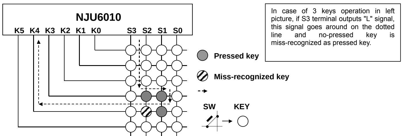
Fig. 7 Multiple Key Inputs
