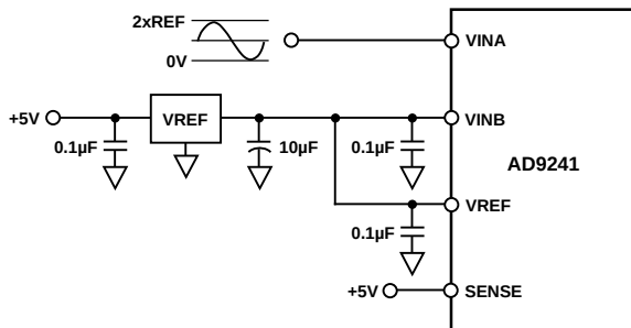
Figure 40. Input Range = 0\text{ V} to 2 \times V_{REF}
