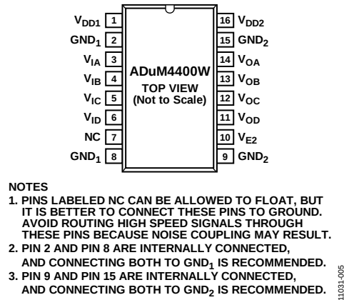
Figure 5. ADuM4400W Pin Configuration
