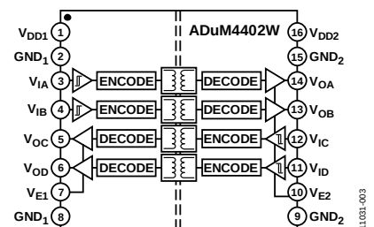
Figure 3. ADuM4402W
