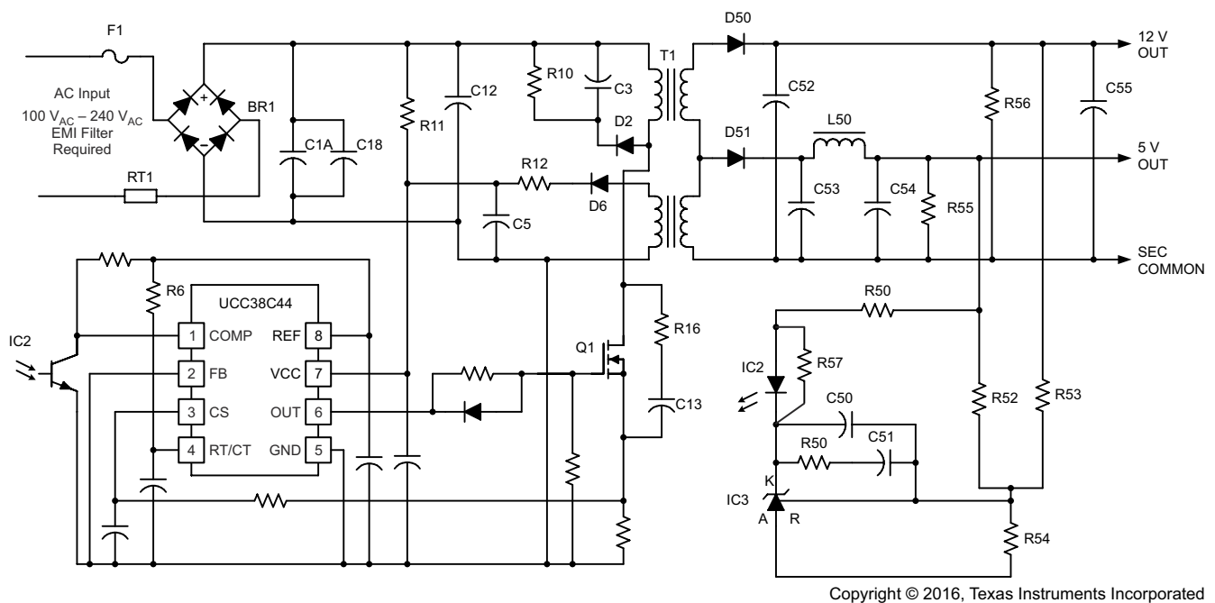
Figure 8-1. Typical Off-Line Application
