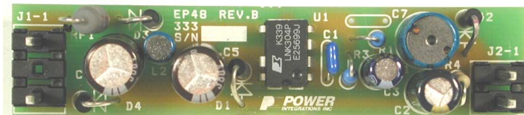
Figure 1 – EP48 Populated Circuit Board Photograph.
