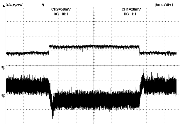
Figure 16 - 265 VAC Input and Maximum Load. Upper: 100 mA / div Lower: 50 mV / div, 5 ms / div
