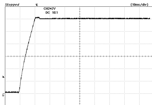
Figure 14 - 265 VAC Input and Maximum Load. 2 V / div, 10 ms
