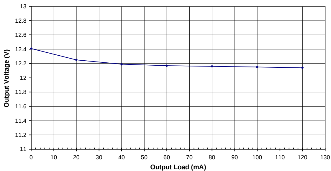
Figure 6 - Load Regulation, Room Temperature.
