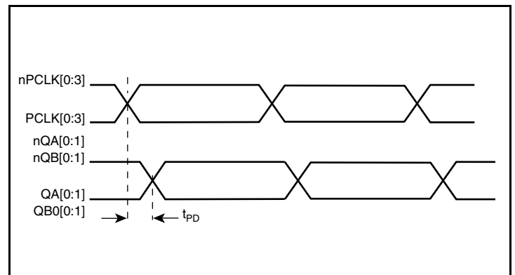
Propagation Delay
