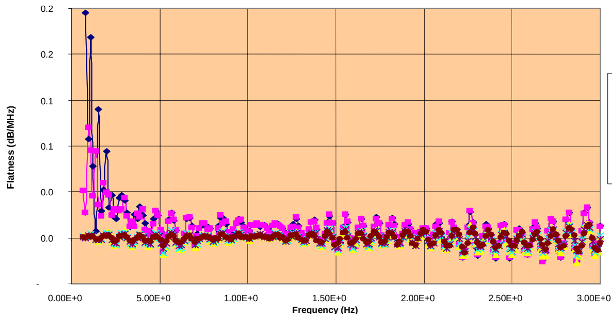
ATTENUATION FLATNESS vs. FREQUENCY
