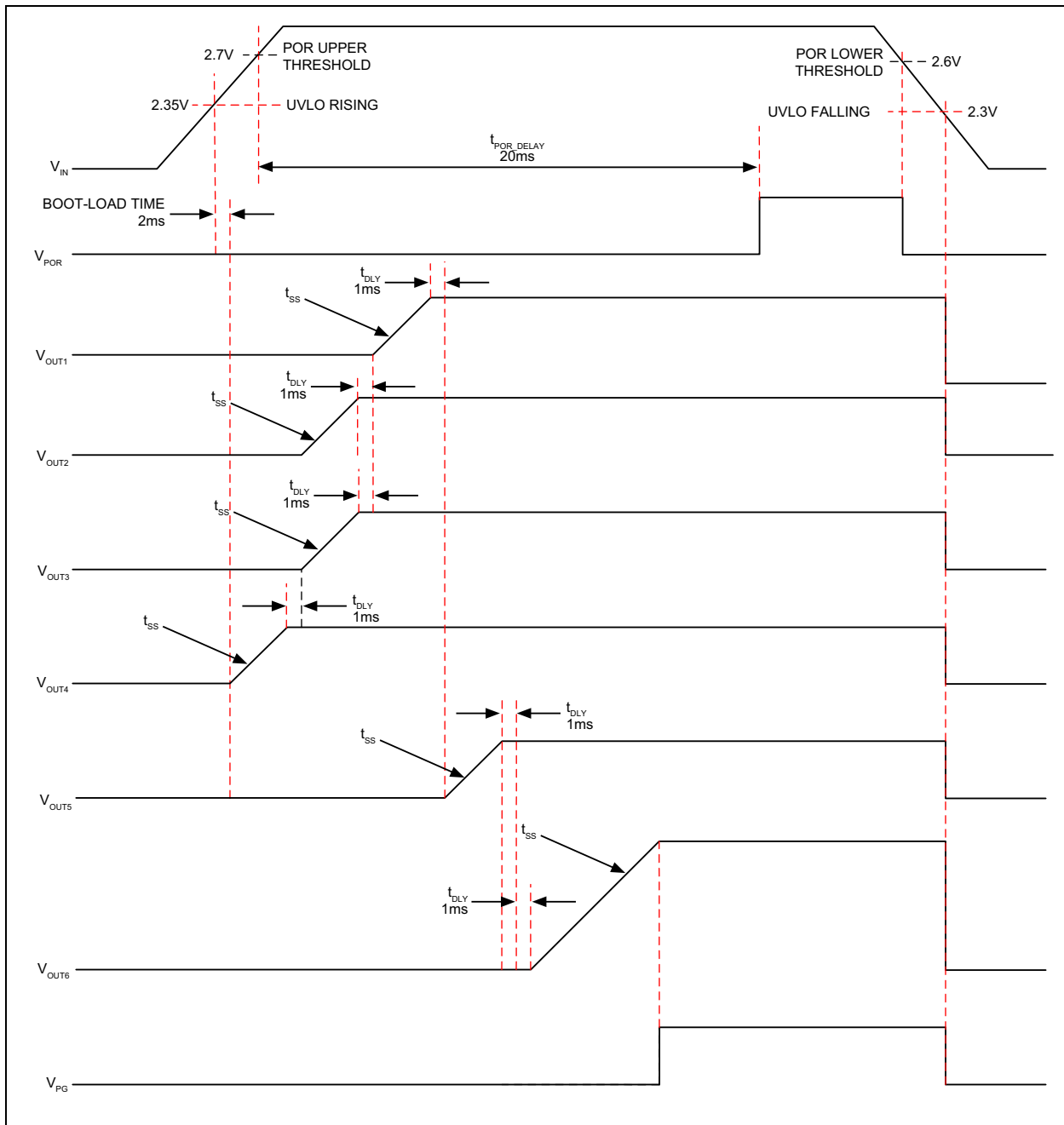
FIGURE 5-1: MIC7400 Power-Up/Down.
