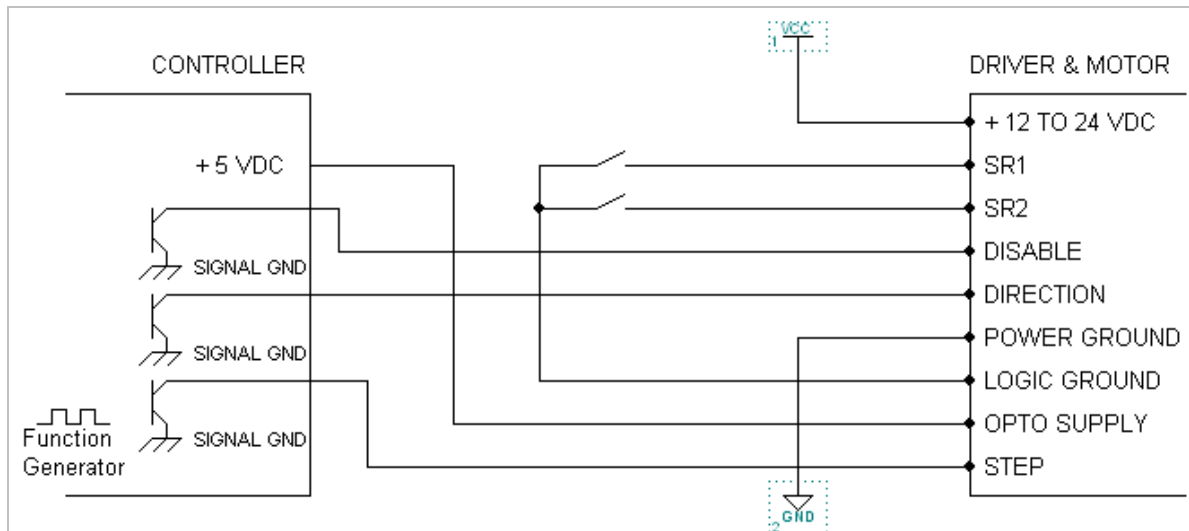
Figure 4: Connections Diagram
