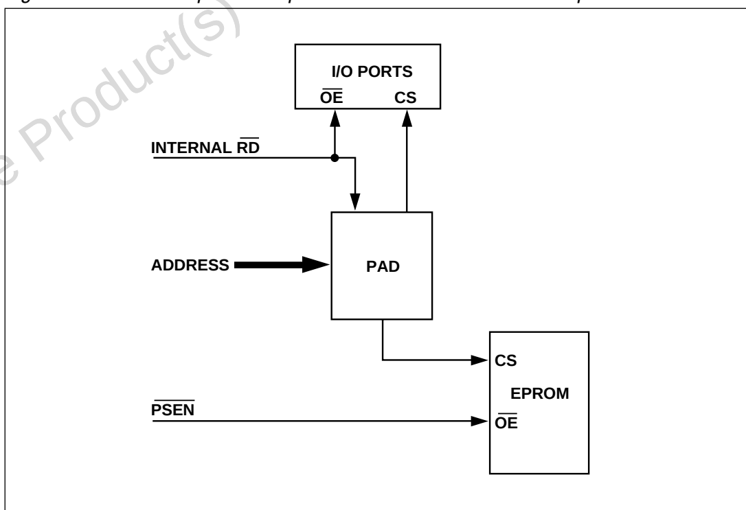
Figure 10. 8031-Compatible Separate Code and Data Address Spaces
