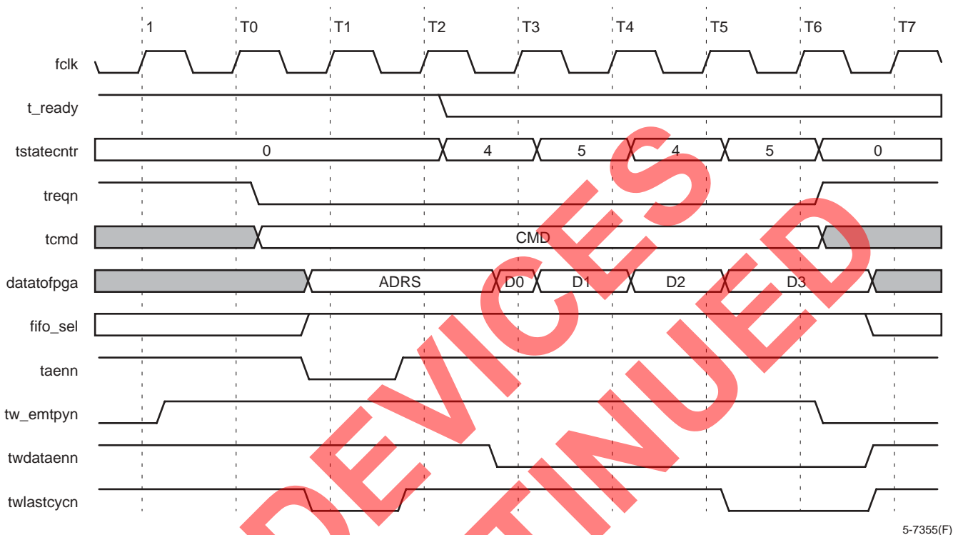
Figure 21. Target Write Burst (FIFO Interface, Dual-Port)
