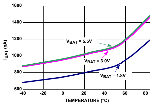
FIGURE 5. I_{BAT} vs TEMPERATURE ( V_{DD} = 0V )
