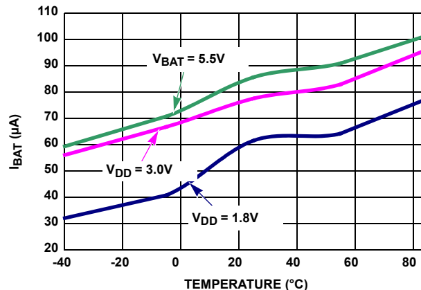
FIGURE 11. I_{BAT} WITH TSE = 1, BTSE = 1 vs TEMPERATURE
