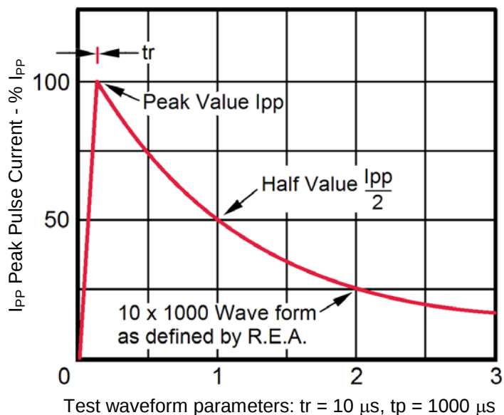
FIGURE 2 Pulse Waveform
