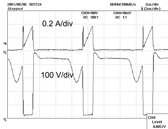
Figure 13 - Drain Current and Drain-to-source Voltage at Full Load ( V_{IN} = 265 VAC, 60 Hz).
