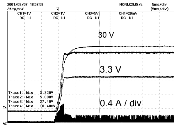
Figure 15 - Primary Current and Output Voltages During Start-up at Minimum Load ( V_{IN} = 265 VAC In, 60 Hz).
