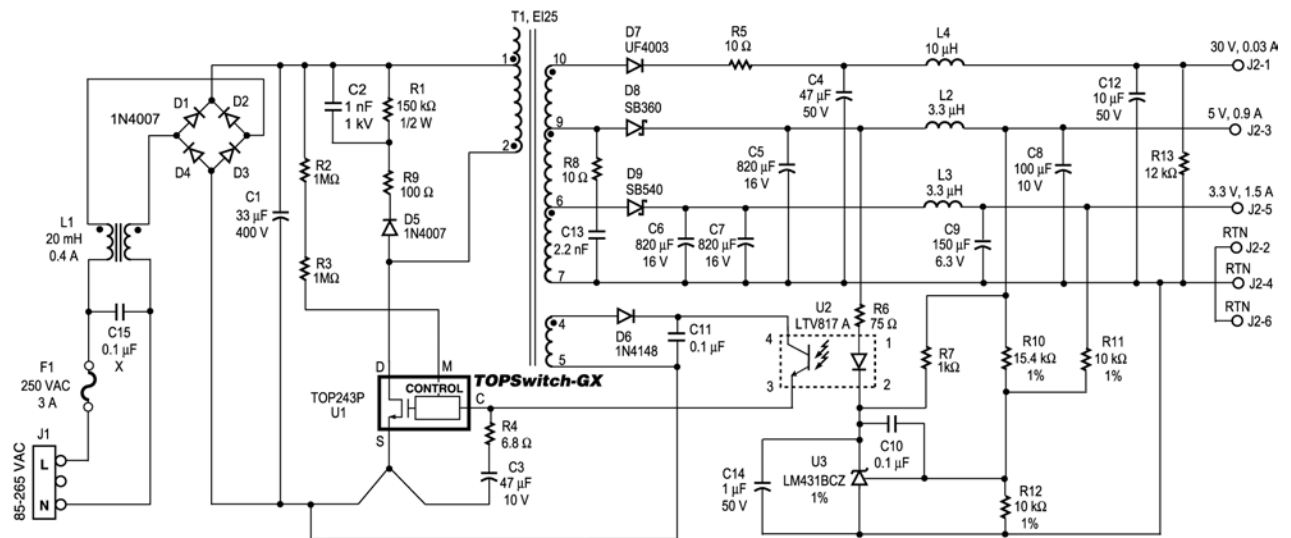
Figure 2 - EP-18 Schematic.
