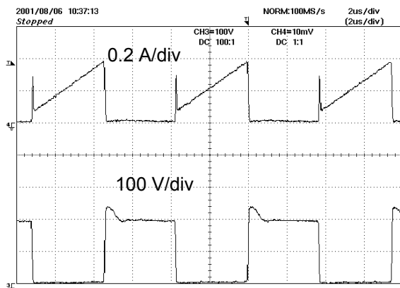
Figure 12 - Drain Current and Drain-to-source Voltage at Full Load ( V_{IN} = 85 VAC, 60 Hz).
