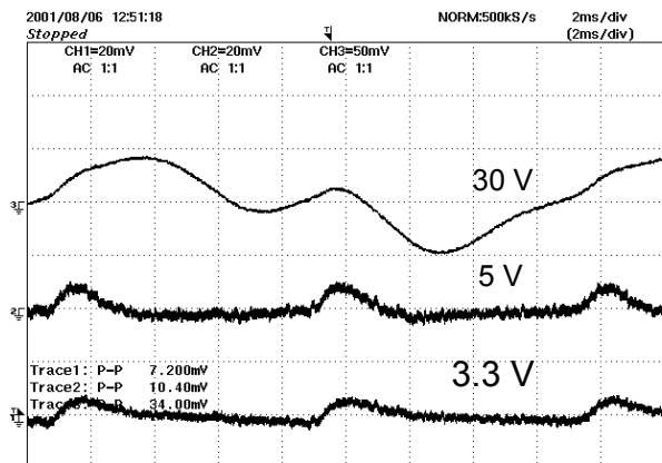
Figure 14 - Output Voltage Ripple at Full Load ( V_{IN} = 85 VAC In, 60 Hz).
