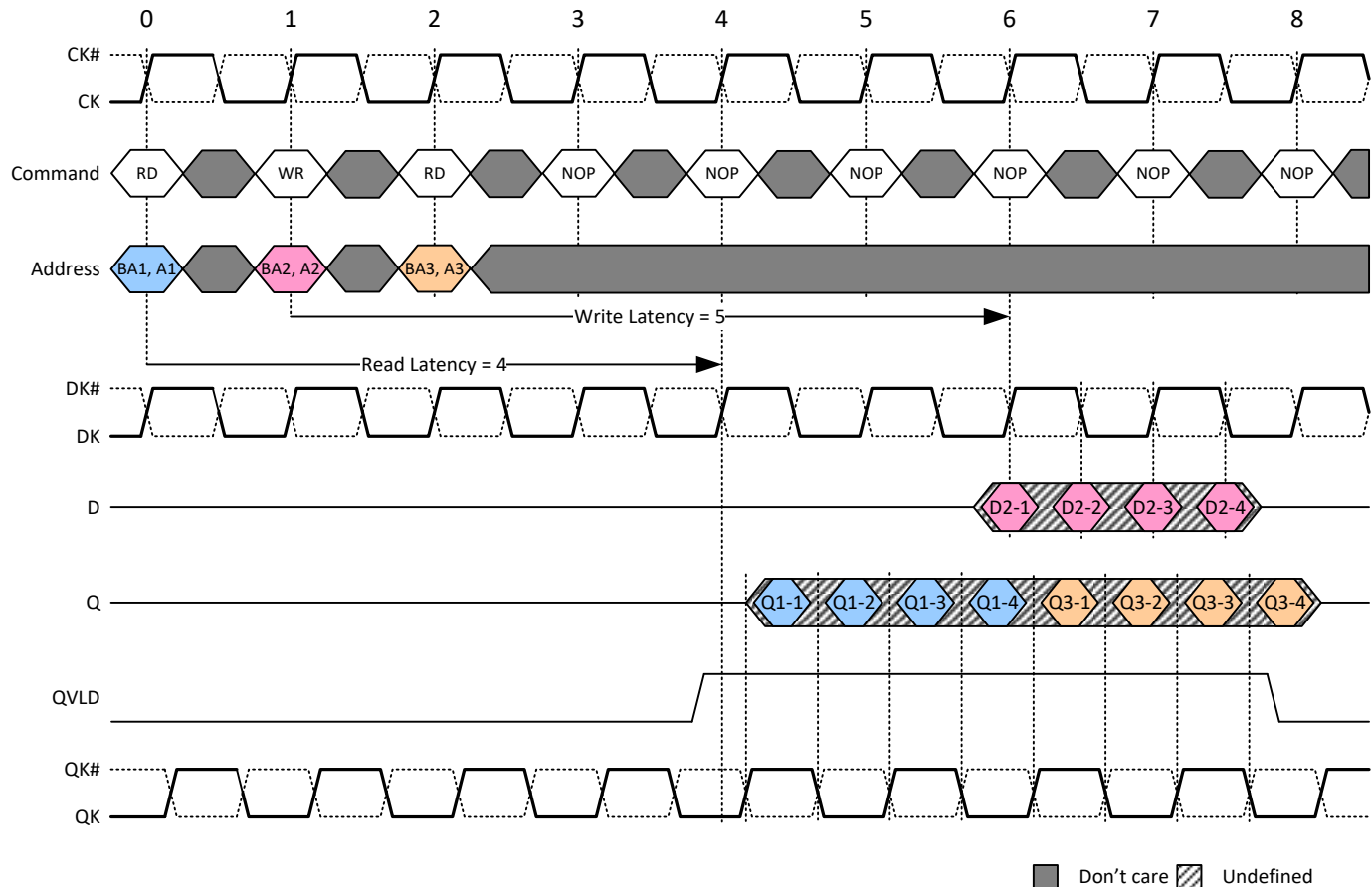
Read Followed by Write: BL = 4, RL = 4 &amp; WL = 5, Configuration 1
