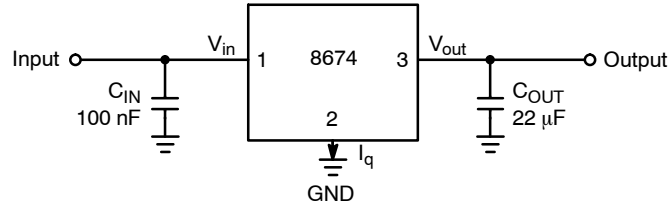
Figure 3. Applications Circuit
