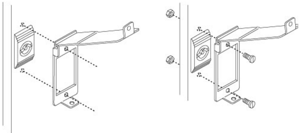
Padlocking Lock System Installation
