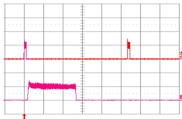
Fig. 12V.18: Load current (top trace, 5 A/div., 20 ms/div.) into a 10 \text{ m}\Omega short circuit during restart, at V_{in} = 24\text{V} . Bottom trace (5 A/div., 1 ms/div.) is an expansion of the on-time portion of the top trace.
