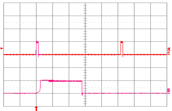
Fig. 3.3V.18: Load current (top trace, 20 A/div., 20 ms/div.) into a 10 \text{ m}\Omega short circuit during restart, at V_{in} = 24\text{V} . Bottom trace (20 A/div., 1 ms/div.) is an expansion of the on-time portion of the top trace.
