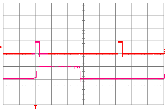
Fig. 1.5V.18: Load current (top trace, 20 A/div., 20 ms/div.) into a 10\ \text{m}\Omega short circuit during restart, at V_{in} = 24\text{V} . Bottom trace (20 A/div., 2 ms/div.) is an expansion of the on-time portion of the top trace.
