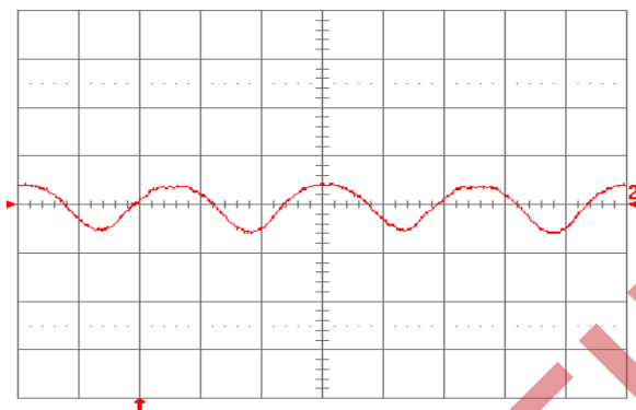
Fig. 1.5V.15: Input reflected ripple current, i_c (100 mA/div.), measured at input terminals at full rated load current and V_{in} = 24\text{V} . Refer to Fig. 1.5V.14 for test setup. Time scale: 1\ \mu\text{s}/\text{div} .
