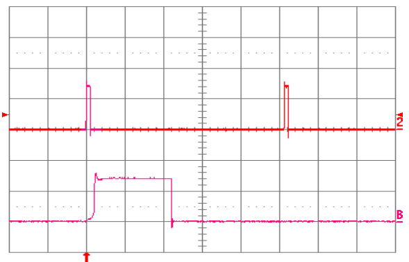
Fig. 5.0V.18: Load current (top trace, 10 A/div., 20 ms/div.) into a 10\ \text{m}\Omega short circuit during restart, at V_{in} = 24\text{V} . Bottom trace (10 A/div., 1 ms/div.) is an expansion of the on-time portion of the top trace.
