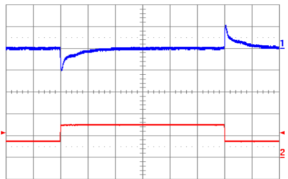
Fig. 3.3V.12: Output voltage response to load current step-change (3.75A – 7.5A – 3.75A) at V_{in} = 24\text{V} . Top trace: output voltage (100 mV/div.). Bottom trace: load current (5 A/div.). Current slew rate: 5 A/ \mu\text{s} . C_o = 450\text{ }\mu\text{F} tantalum + 1 \mu\text{F} ceramic. Time scale: 0.2 ms/div.
