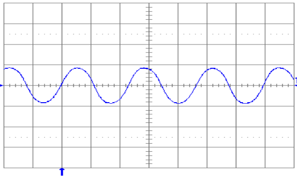
Fig. 12V.13: Output voltage ripple (50 mV/div.) at full rated load current into a resistive load with C_o = 10 \mu\text{F} tantalum + 1 \mu\text{F} ceramic and V_{in} = 24\text{V} . Time scale: 1 \mu\text{s}/\text{div} .
