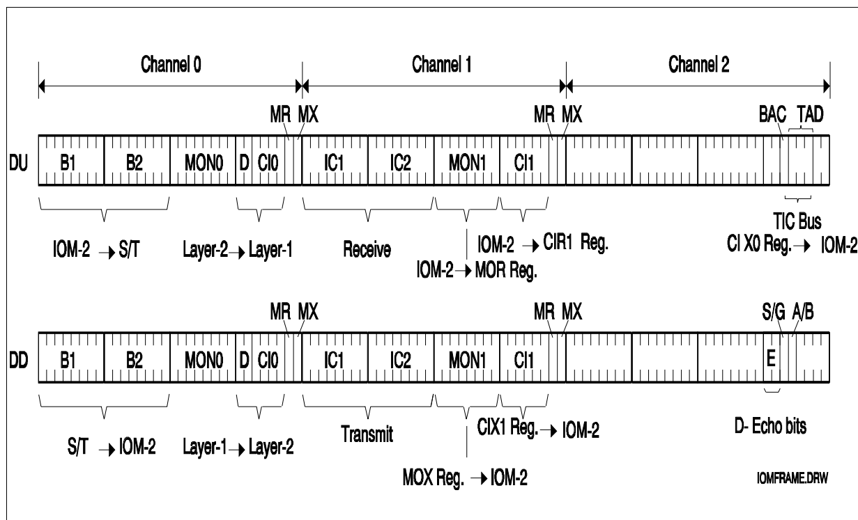
Figure 40 IOM ® -2 Frame Structure in Terminal Mode
