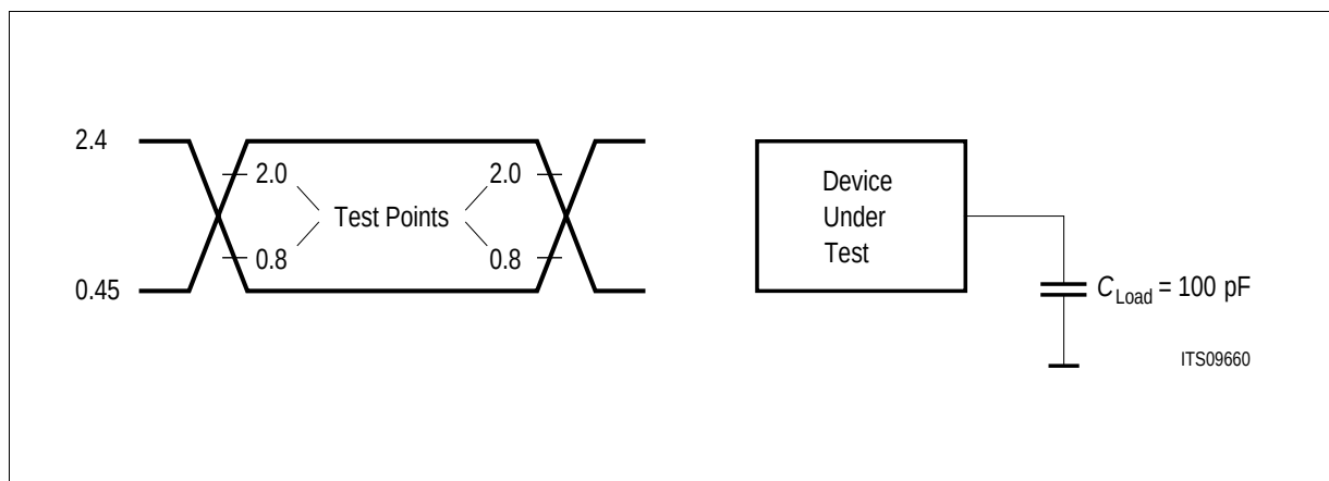
Figure 68 Input/Output Waveform for AC Tests
