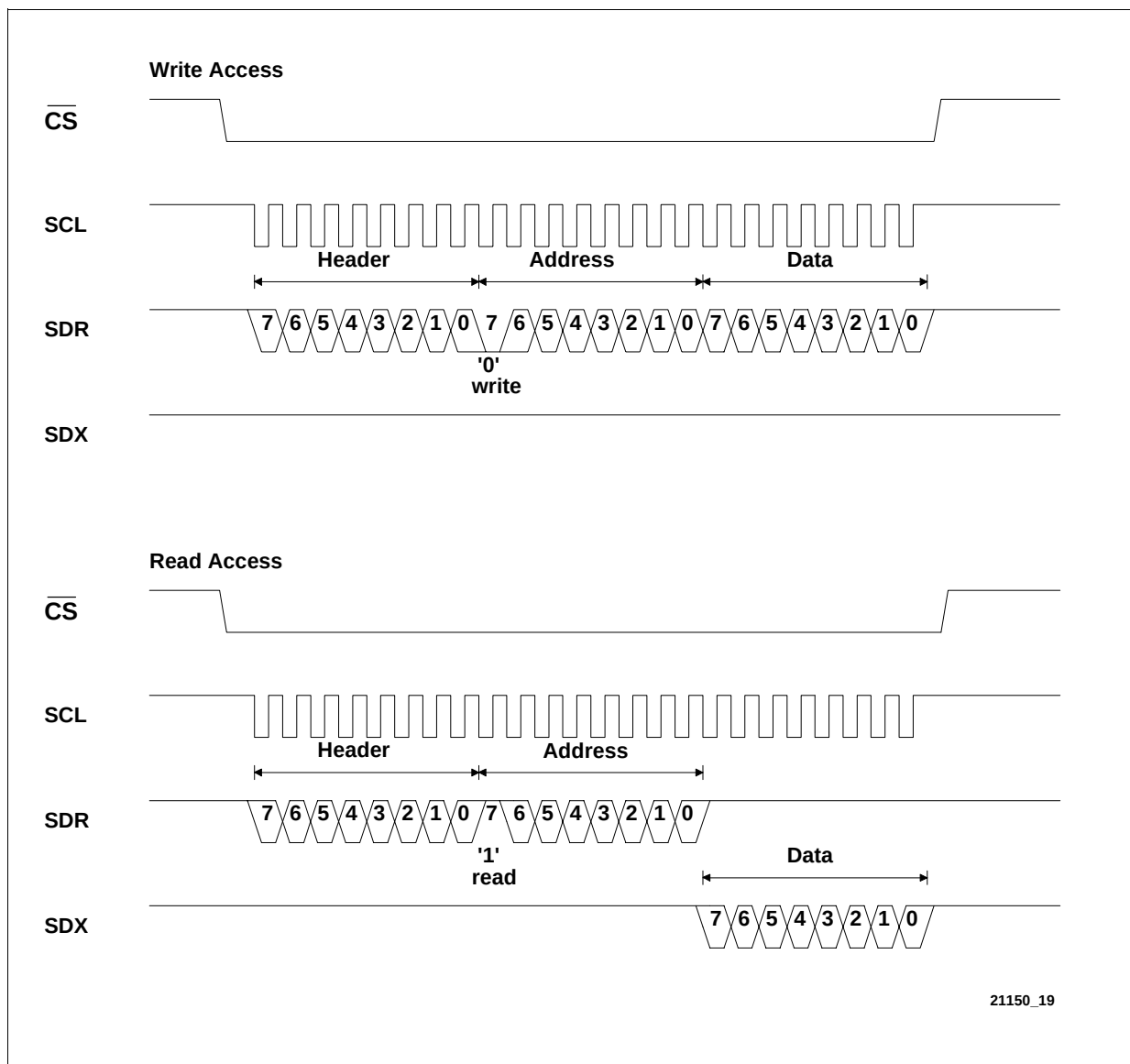
Figure 6 Serial Control Interface Timing
