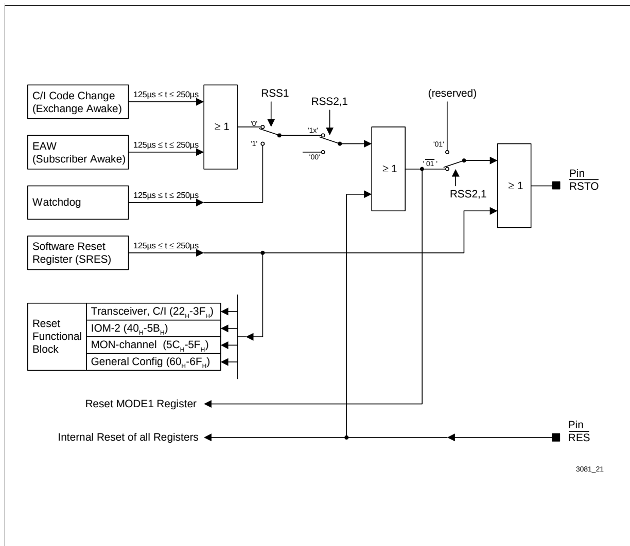
Figure 9 Reset Generation
