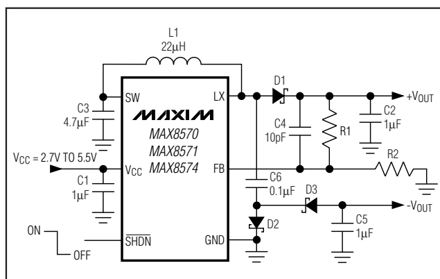
Figure 5. Negative Output Voltage for LCD Bias
