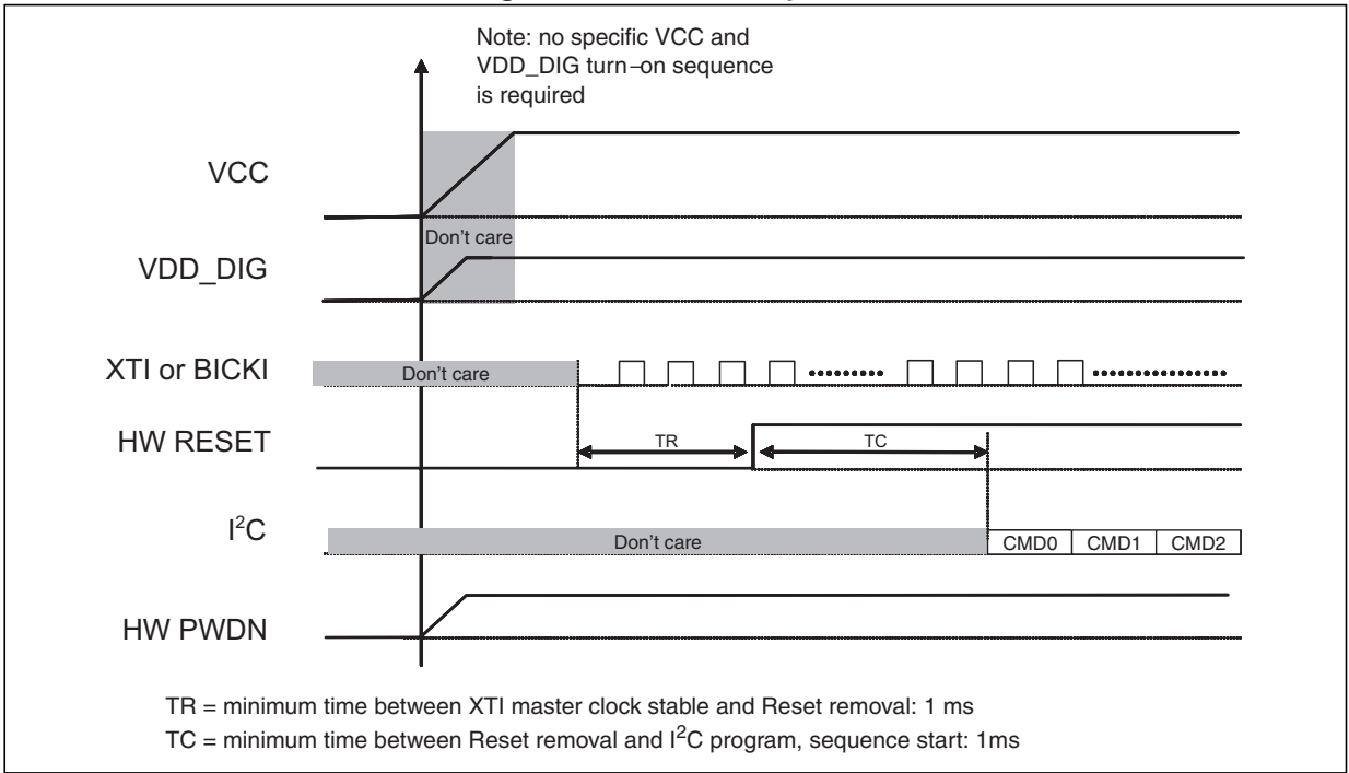
Figure 4. Power-on sequence
