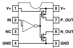
EL7104 (8-PIN SO, PDIP) TOP VIEW
