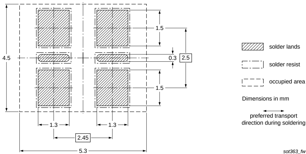
Fig 20. Wave soldering footprint PUMD48 (SOT363/SC-88)
