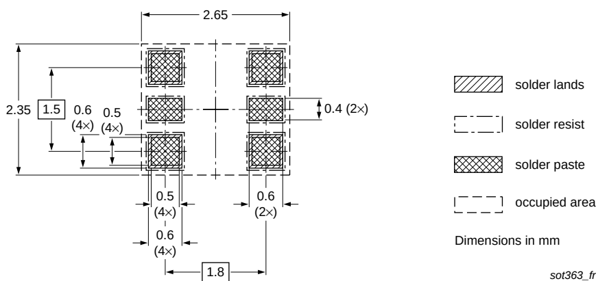
Fig 19. Reflow soldering footprint PUMD48 (SOT363/SC-88)
